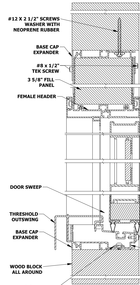
SECTION B-B
